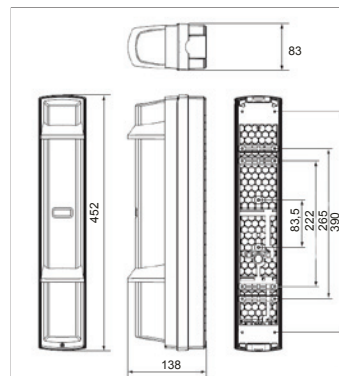
Obr. 10: Dimensions of units
